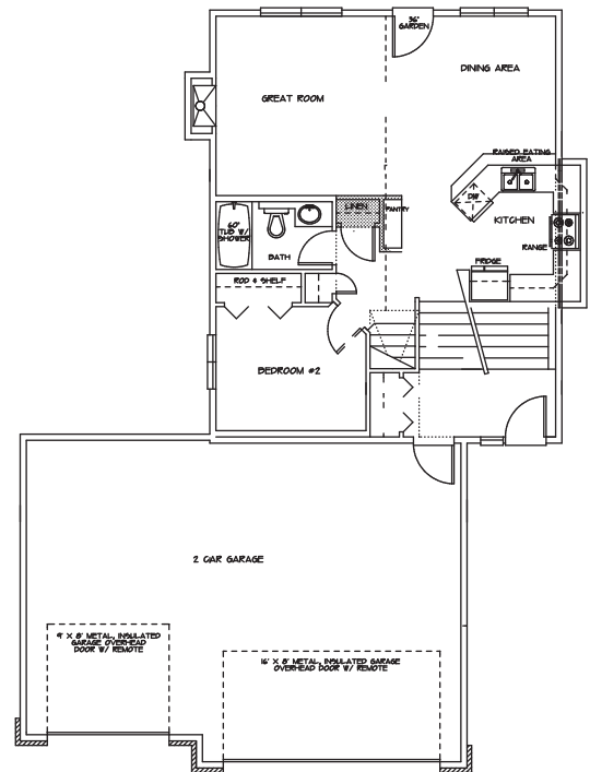
MAIN FLOOR PLAN 852 SQ. FT.
