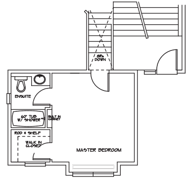
TOP FLOOR PLAN 277 SQ. FT.
