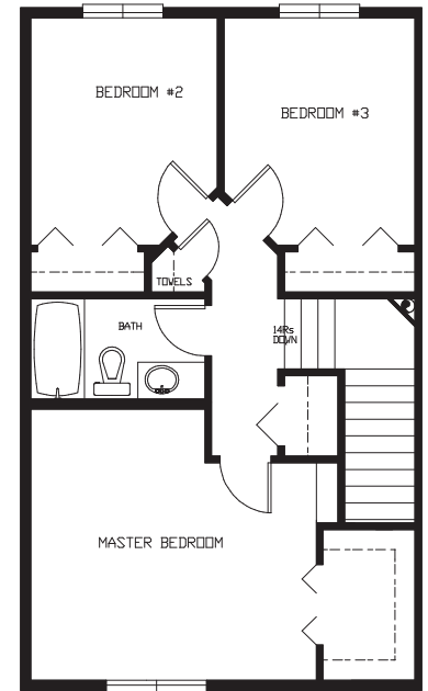
TOP FLOOR 681 SQ. FT.
