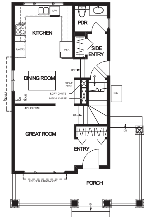
MAIN FLOOR PLAN 561 FEET SQ.
