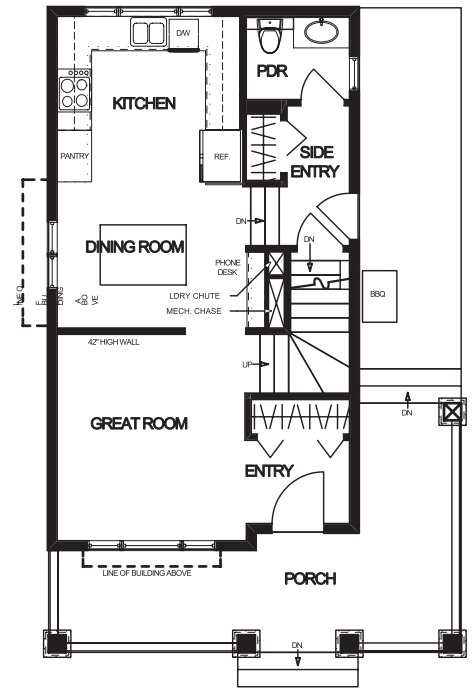
MAIN FLOOR PLAN 561 FEET SQ.
