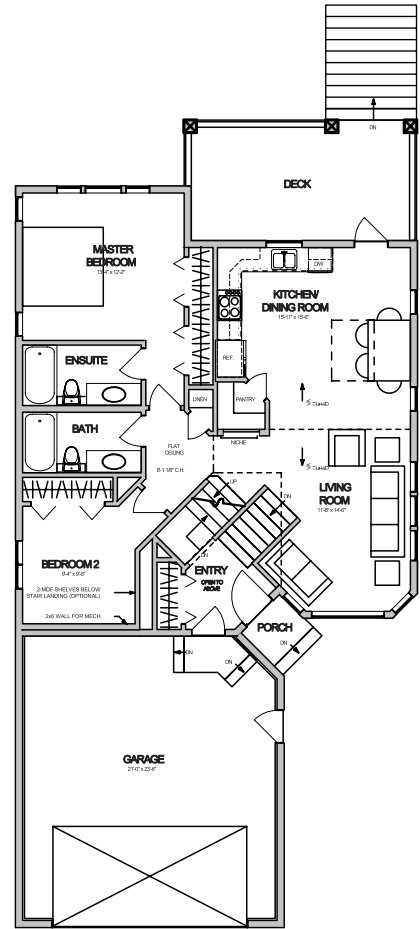
MAIN FLOOR PLAN 1110 FEET SQ.
