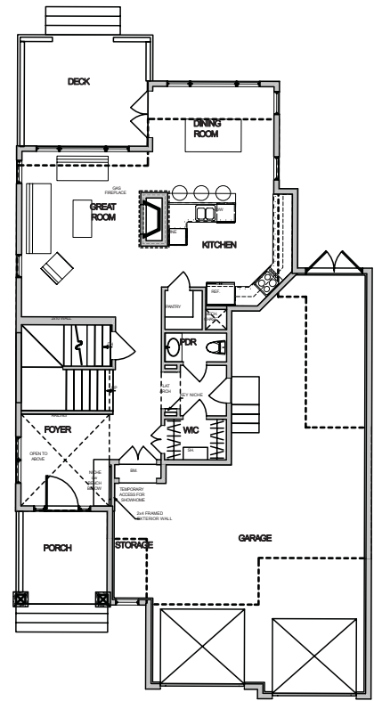
MAIN FLOOR PLAN 1062 FEET SQ.
