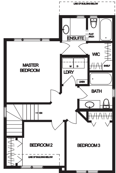
UPPER FLOOR PLAN 720 FEET SQ.
